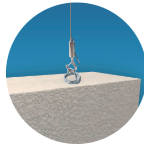
System No. 101 (H/V) (Soft Hanging System) Spiral Pin + Adjustable Hanging Wire
