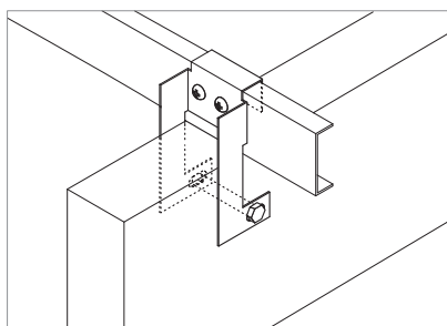
System No. 201 (V) (Hard Hanging System) Pacifico Method
