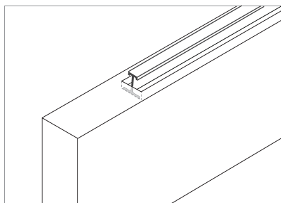
System No. 203 (V) Built-in Aluminum Rail(s) Fixed with Glue and Screws
